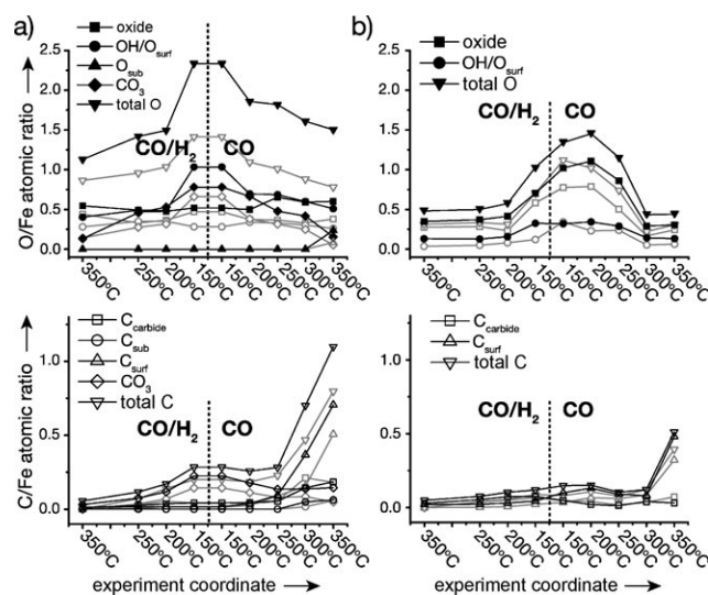
Figure 3. O/Fe and C/Fe ratios for various species during the \text{CO}/\text{H}_2 and CO treatment at various temperatures. a) Nanoparticulate iron oxide and b) bulk iron oxide. Black symbols indicate ratios at 7 Å IMFP, gray symbols indicate ratios at 11 Å IMFP.
